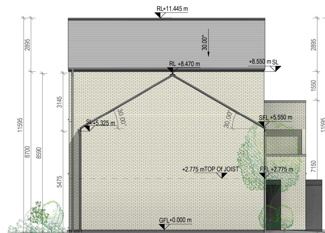
4 Side Elevation 2 1 : 100
